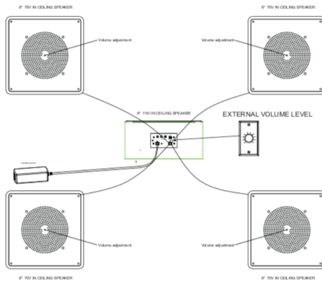
CMA225+CSQ8VR Sound Masking system
